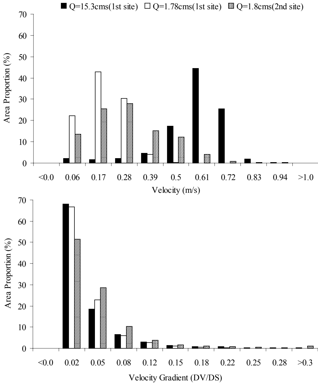
Figure 12. Velocity (m/s) and velocity gradient (DV/DS) at 4.2 km (1 st site) and 12.6 km (2 nd site) below Philpott dam, Smith River, Virginia at discharges of 15.3 and 1.78 m 3 /s (1 st site), and 1.8 m 3 /s (2 nd site).
