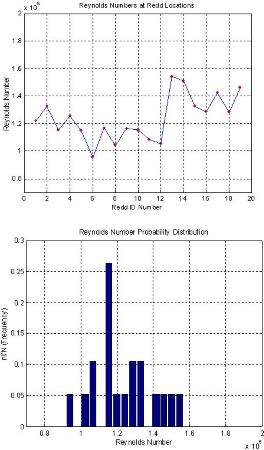
Figure 10. Calculated reynolds number and frequency distribution at selected redd locations in the site 4.2 km below Philpott dam, Smith River, Virginia at a discharge of 1.83 \text{ m}^3/\text{s} .
