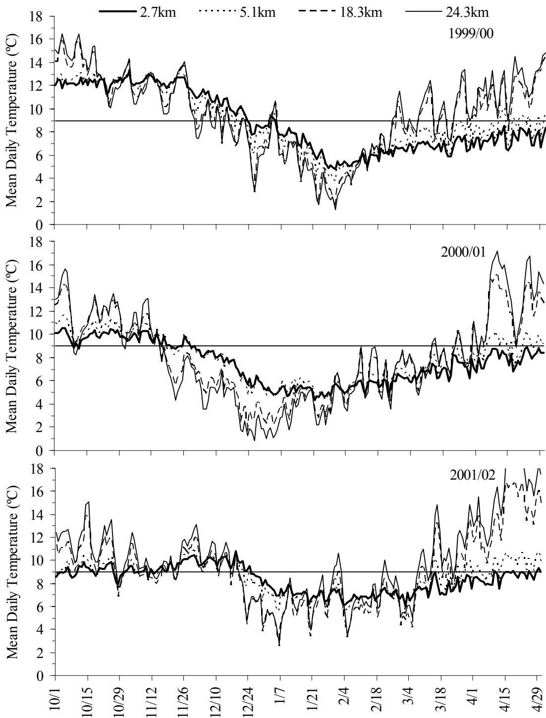
Figure 2. Mean daily water temperature (°C) during brown trout spawning, incubation, and emergence period at 2.7, 5.1, 18.3, and 24.3 km below Philpott dam in the Smith River, VA during 1999/00, 2000/01, and 2001/02. Horizontal line displays 9°C, which is the temperature believed to initiate spawning.
