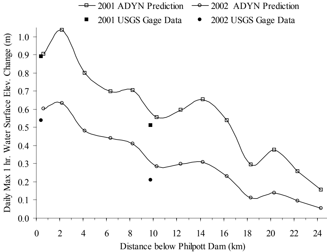
Figure 9. Daily maximum hourly water surface elevation change (m) averaged from March 15 to April 23 for 2001 and 2002 (excluding non-generation weekends) at 2 km intervals below Philpott dam for ADYN model predictions and USGS gage data. Data derived from ADYN hydraulic model predictions assumed lateral inflow to be constant representative flows over the predicted time period.
