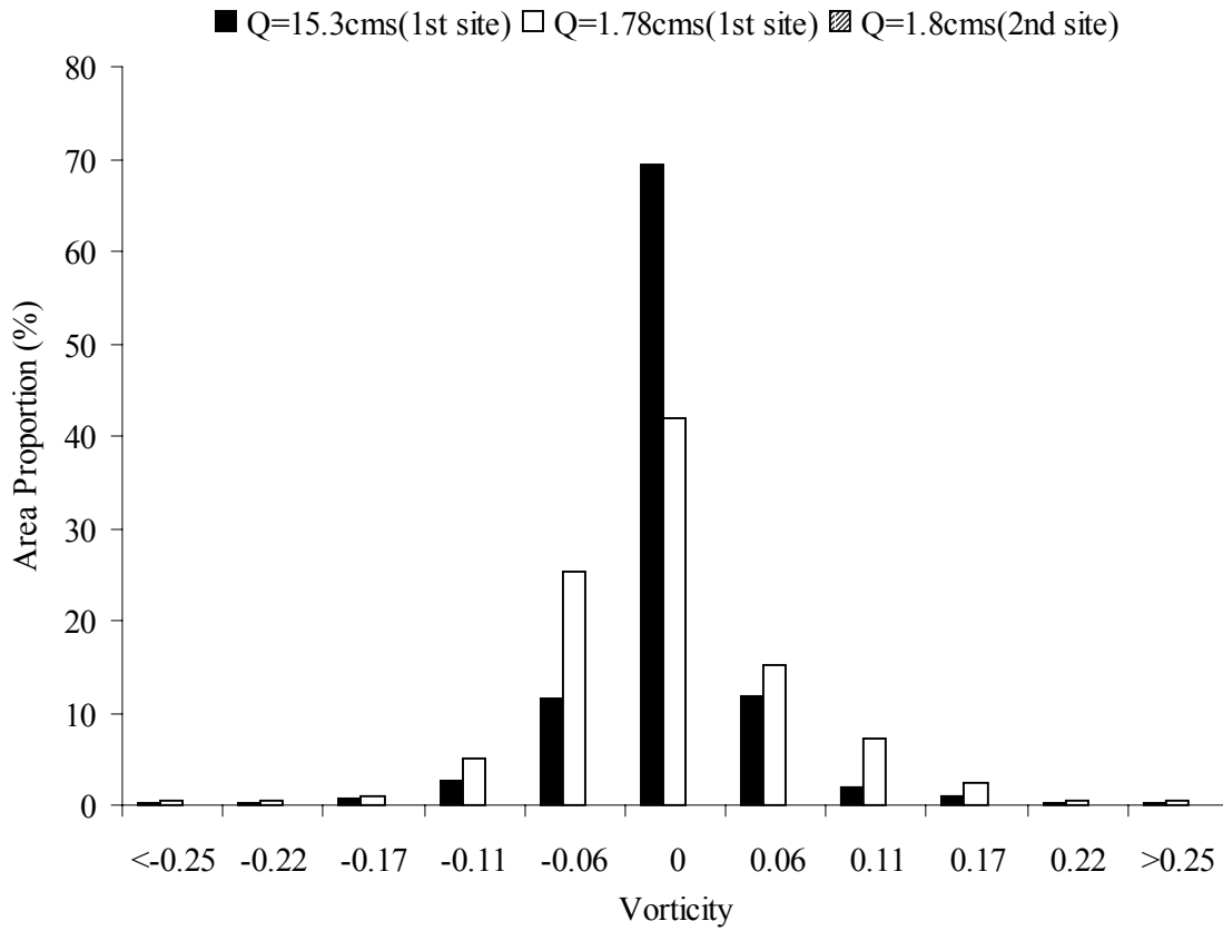
Figure 14. Vorticity at 4.2 km (1 st site) and 12.6 km (2 nd site) below Philpott dam, Smith River, Virginia at discharges of 15.3 and 1.78 m 3 /s (1 st site), and 1.8 m 3 /s (2 nd site).
