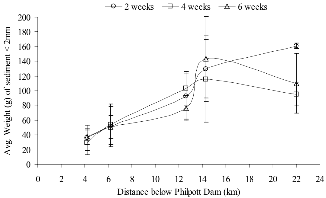
Figure 11. Average weight (g) of sediment <2 mm intruded over 2, 4, and 6 weeks (summer 2002) into vibert boxes at 4.2, 6.2, 12.6, 14.3, and 22.0 km below Philpott dam, Smith River, VA. Error bars represent \pm 2SE .
