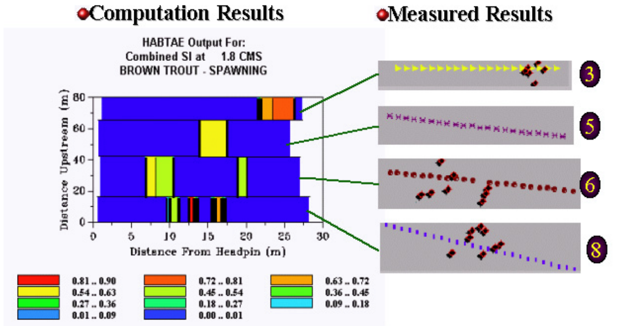
Figure 7. Computation results compared with field data shows the location of redds.
