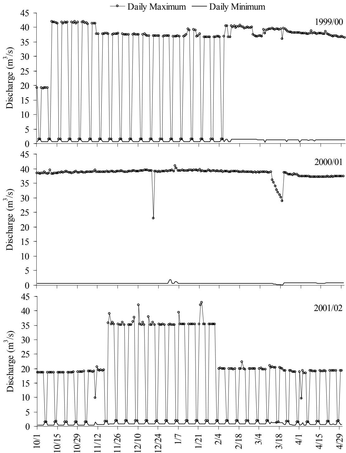
Figure 3. Daily maximum and minimum discharge ( \text{m}^3/\text{s} ) during brown trout spawning, incubation, and immergence period at 0.5 km below Philpott dam in the Smith River, VA during 1999/00, 2000/01, and 2001/02.
