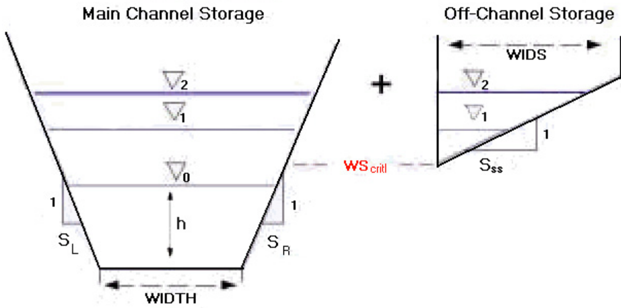
Figure 4. A representative cross section of channel storage and off-channel storage.
