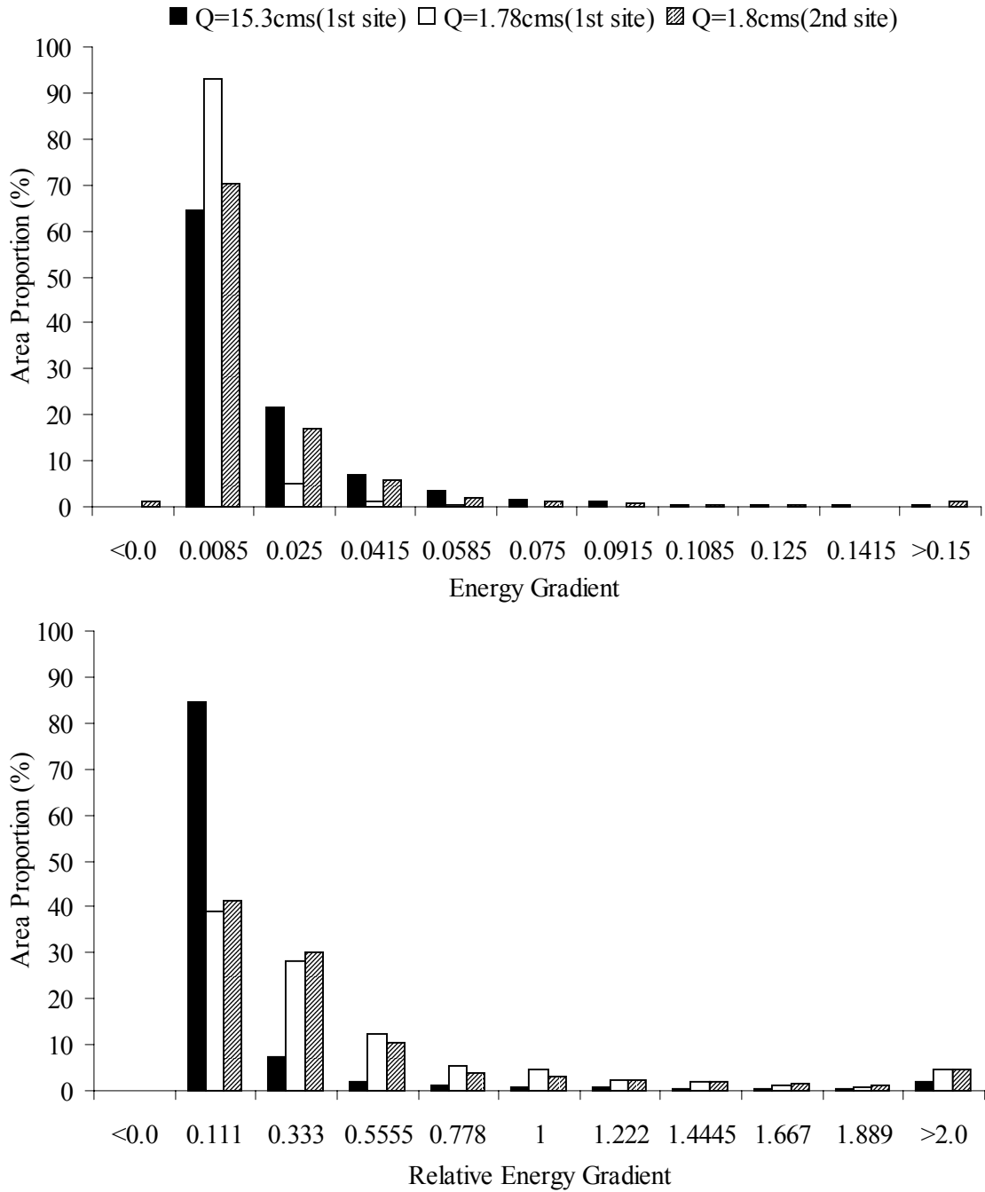
Figure 13. Energy gradient and relative energy gradient at 4.2 km (1 st site) and 12.6 km (2 nd site) below Philpott dam, Smith River, Virginia at discharges of 15.3 and 1.78 m 3 /s (1 st site), and 1.8 m 3 /s (2 nd site).
