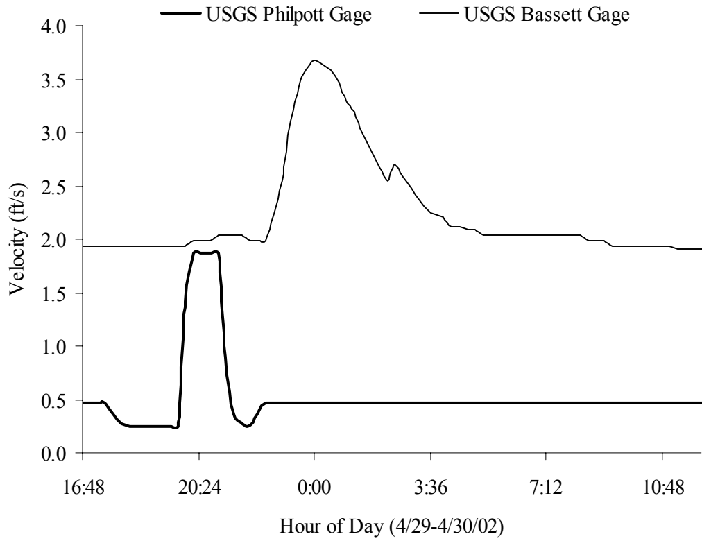
Figure 3. Typical velocity hydrographs from Philpott & Bassett USGS gage stations, Smith River, Virginia.
