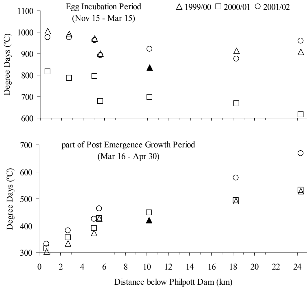
Figure 4. Degree days ( ^{\circ}\text{C} ) (sum of daily mean water temperature) at 0.7, 2.7, 5.1, 5.6, 10.2, 18.3, and 24.3 km below Philpott dam in the Smith River, VA during the typical egg incubation period (11/15 - 03/15) and part of the growth period after emergence (03/16 - 04/30) during 1999/00, 2000/01, and 2001/02. Open symbols represent data logger recorded data and solid symbols represent model (RQUAL) predict values where logger data is missing. Data is currently unavailable for the 2001/02 post emergence period.
