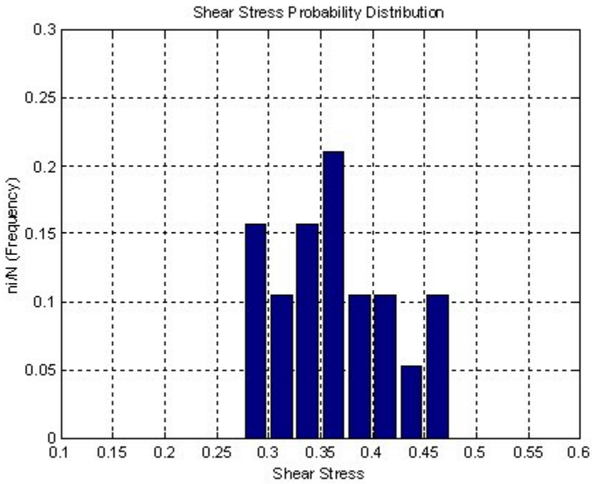
Figure 11. Calculated shear stress and frequency distribution at selected redd locations in the site 4.2 km below Philpott dam, Smith River, Virginia at a discharge of 1.83 \text{ m}^3/\text{s} .
