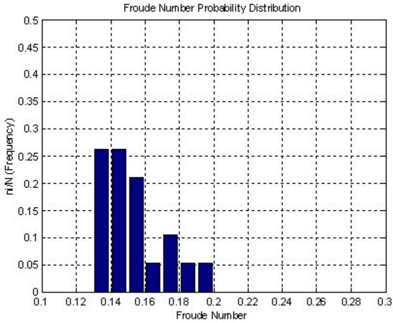
Figure 9. Calculated Froude number and frequency distribution at selected redd locations in the site 4.2 km below Philpott dam, Smith River, Virginia at a discharge of 1.83 \text{ m}^3/\text{s} .
