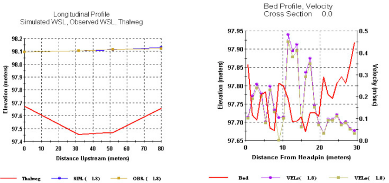
Figure 5. Simulated water surface elevation (WSL), measured WSL, simulated velocities, and observed velocity distribution along transect #8 (Figure 1) at 4.2 km below Philpott dam, Smith River, Virginia.
