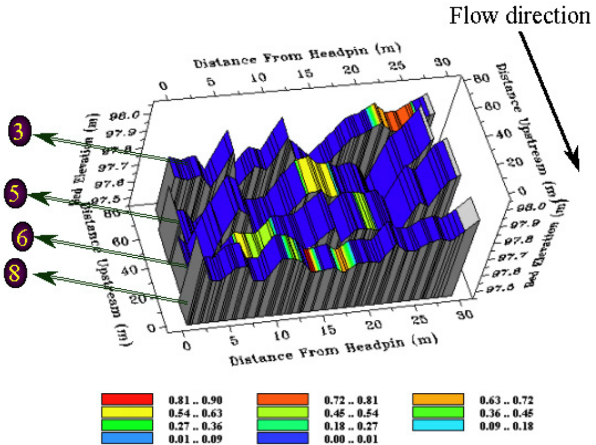
Figure 6. HABTAE output for combined suitability indexes (0.0 ~ 1.0) at 1.8 \text{ m}^3/\text{s} for brown trout at spawning life stage. HABTAE is a model of PHABSIM, which allows integration of biological requirement of target species and life stages represented in the form of HSC with hydraulic simulation results to generate a number of indices of available habitat quantity and quality
