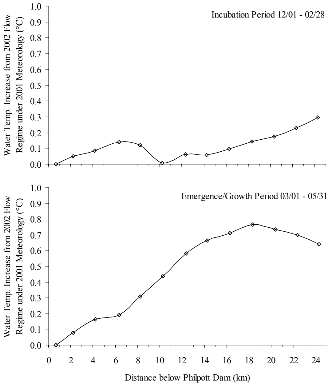
Figure 10. Average change in water temperature (°C) predicted with the ADYN & RQUAL model if the 2002 Smith River flow regime occurred during 2001 (i.e., under 2001 meteorological conditions). This modeling exercise shows that the 2002 flow regime produces warmer water temperatures than the 2001 flow regime regardless of meteorological conditions.
